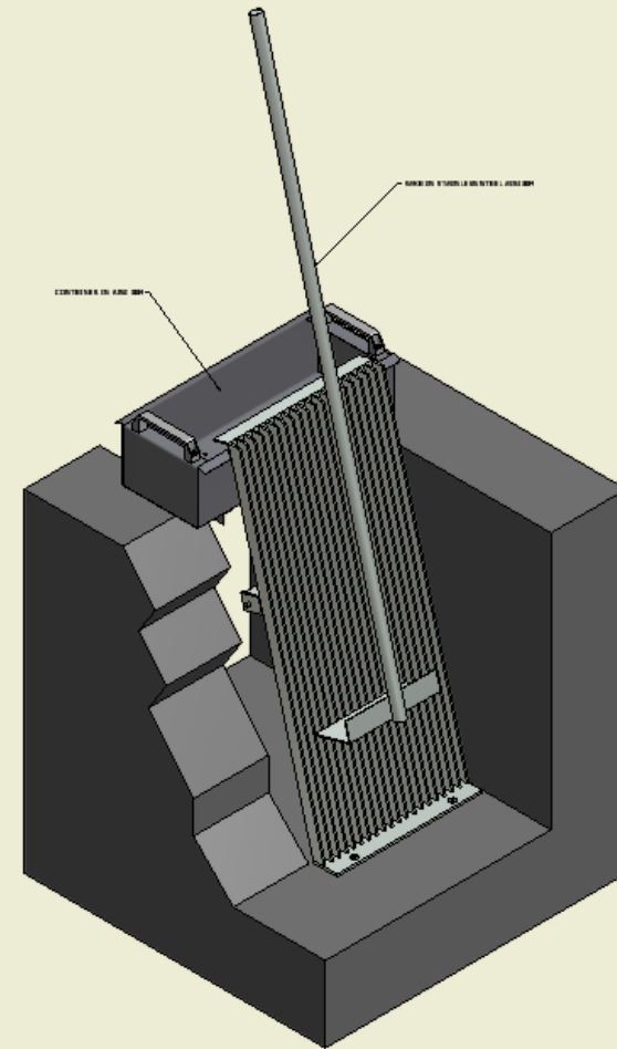
ISOMETRIC VIEW SCALE ( 1 : 4 )
