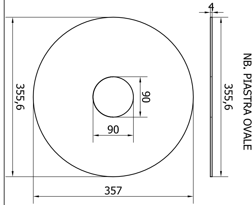
POS.15 SCALA ( 1:5 )
